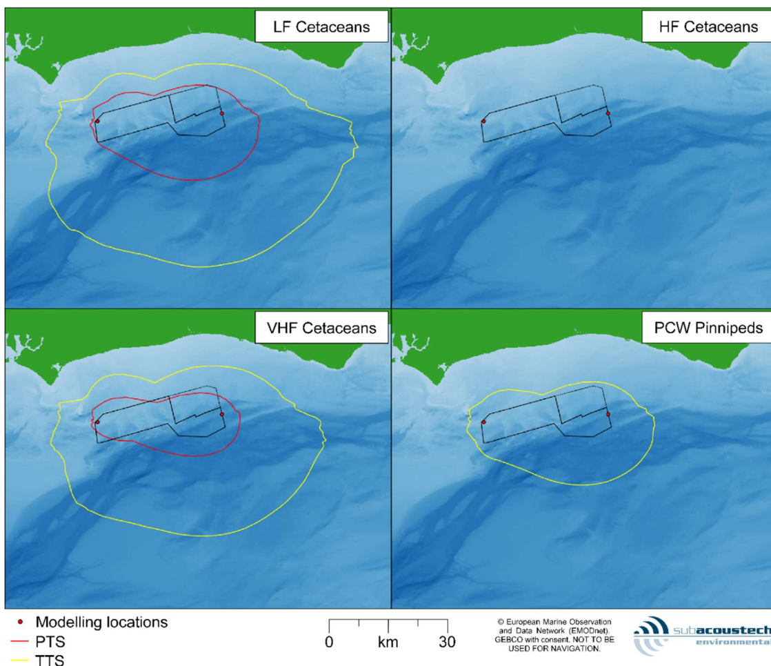
Figure 4-5 Contour plots showing the in-combination impacts of simultaneous installation of worst-case jacket pile foundations (based on 4 piles installed sequentially) at the E and W modelling locations for marine mammals using the Southall et al. (2019) impulsive criteria, assuming a fleeing receptor
