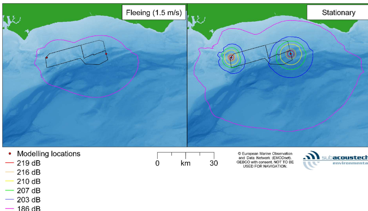
Figure 4-9 Contour plots showing the in-combination impacts of simultaneous installation of worst-case jacket foundations (based on 4 piles installed sequentially) at the E and W modelling locations for fish using the Popper et al. (2019) impact piling criteria, assuming fleeing and stationary receptors
